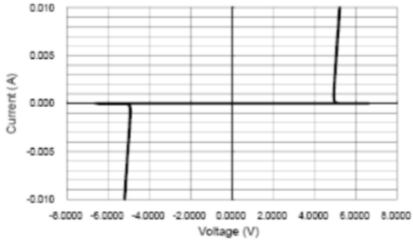
FIGURE 3 Voltage Sweeping
